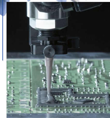
Dam&Fill-coating is key for encapsulation and thick layer PCB protection. Whatever protection you need – it can be done with BECTRON®
