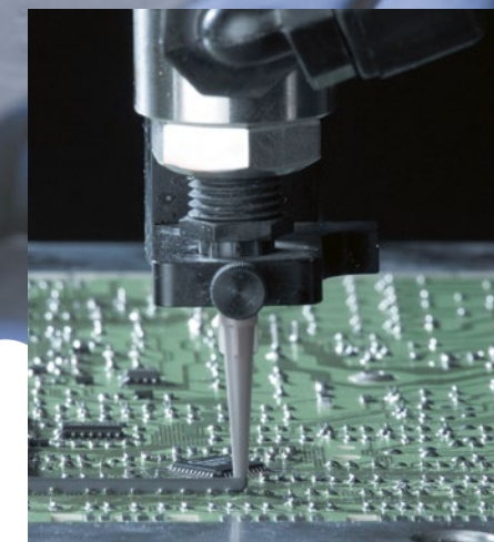
Dam&Fill-coating is key for encapsulation and thick layer PCB protection. Whatever protection you need – it can be done with BECTRON®
